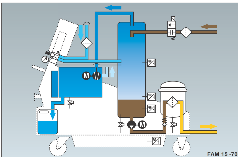
FluidAqua Mobil FAM 50
