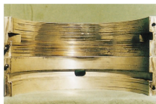
Lagerverschleiß Bearing wear & tear/ Friction bearing Usure de roulements / Palier lisse
